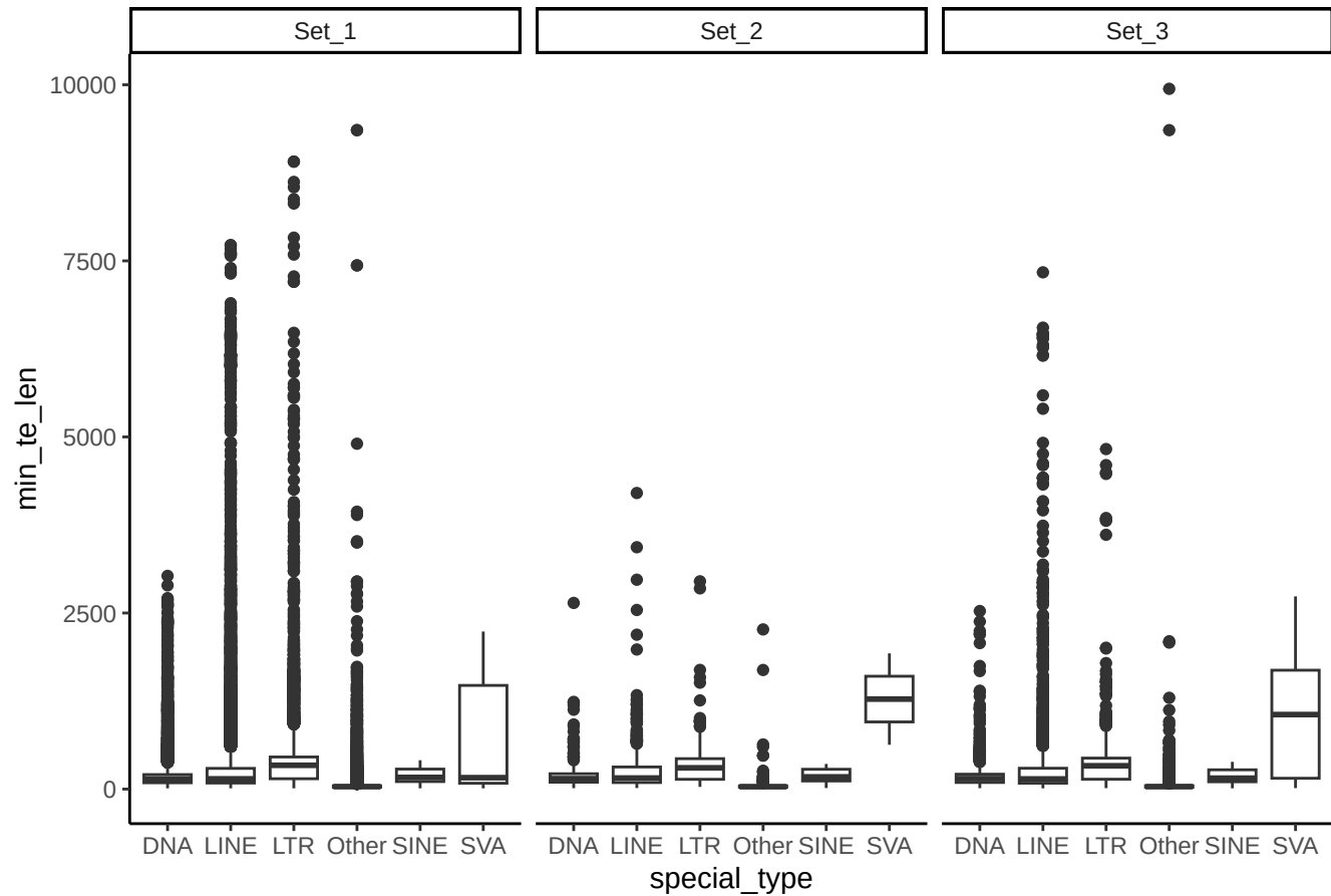
Overlapping minimum TE length per class in H3K27ac
